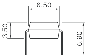
DIP Type
