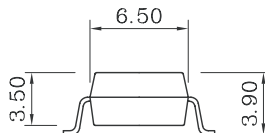
SMD Type
