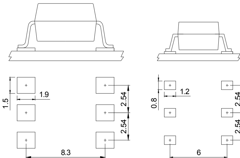
6-pin SMD
