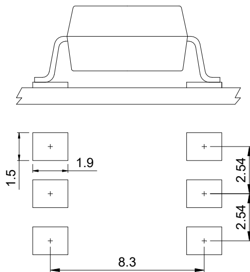
6-pin SMD
