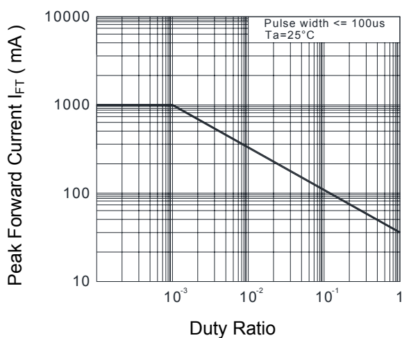
Fig.5 Peak Forward Current I_{FT} vs. Duty Ratio
